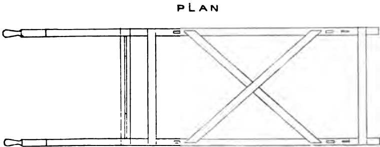
PLATE III. HIMALAYAN SLEDGE FOR RAILWAY SLEEPERS.
